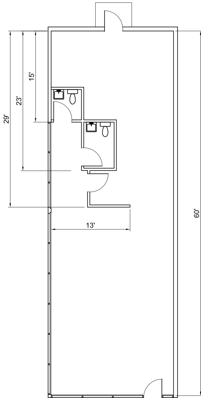
Floor Plan Suite D - 1 1,200 SF
