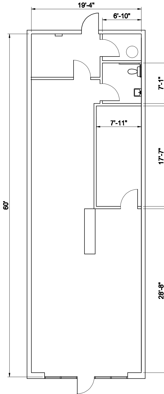
Floor Plan Suite 30 No Scale 1,200 SF
