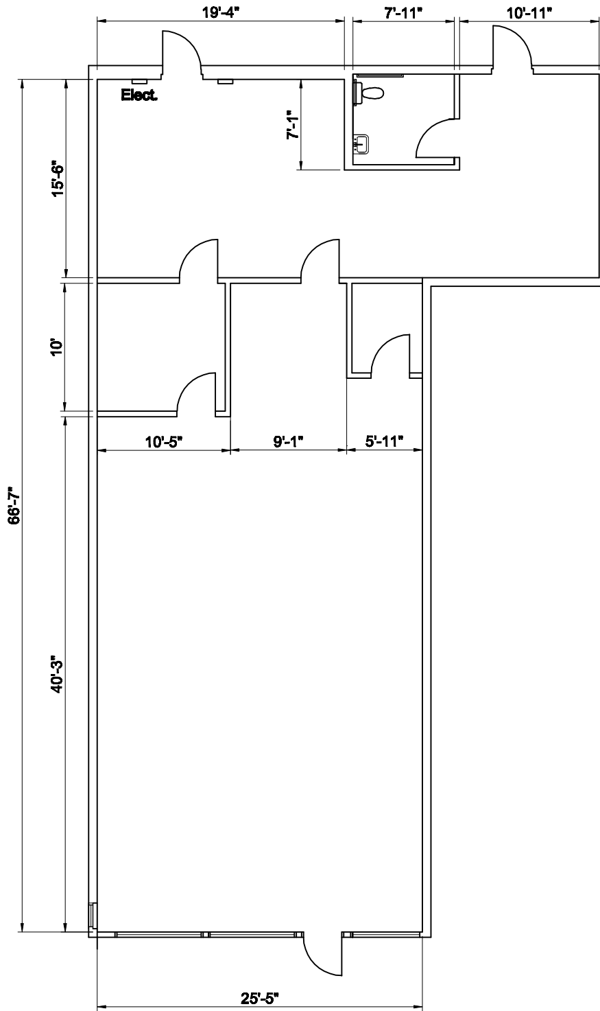
Floor Plan Suite 11 No Scale 2,000 SF
