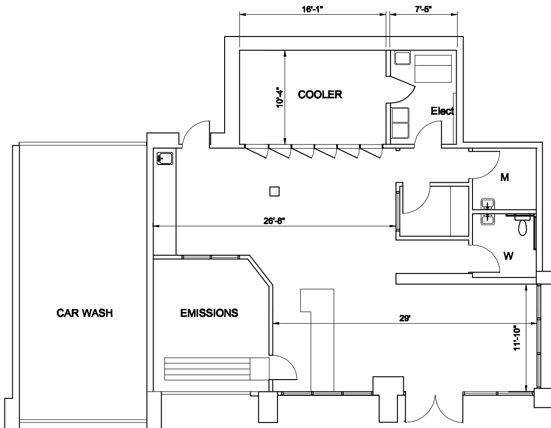
Floor Plan No Scale 2,400 SF
